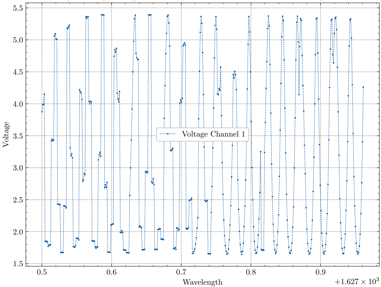
Voltage Data (0, 9999) LUT Extrapolated with 3 Intermediate Integer Values
